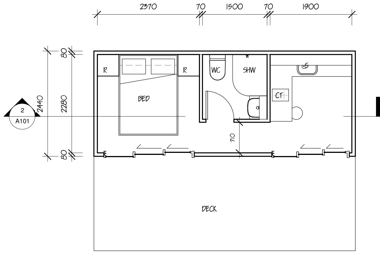
1 Ground Floor 1:50
